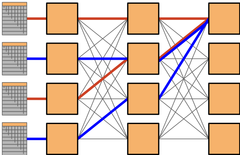
Per-flow load balancing might cause 2 elephant flows to share a link.
